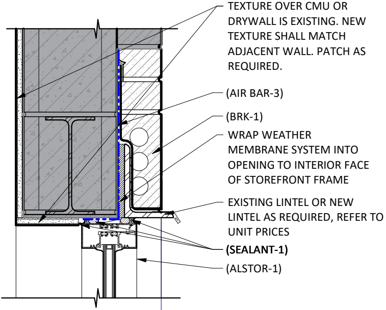
4A A311 BRICK HEAD DETAIL SCALE: 1 1/2" = 1'-0"
