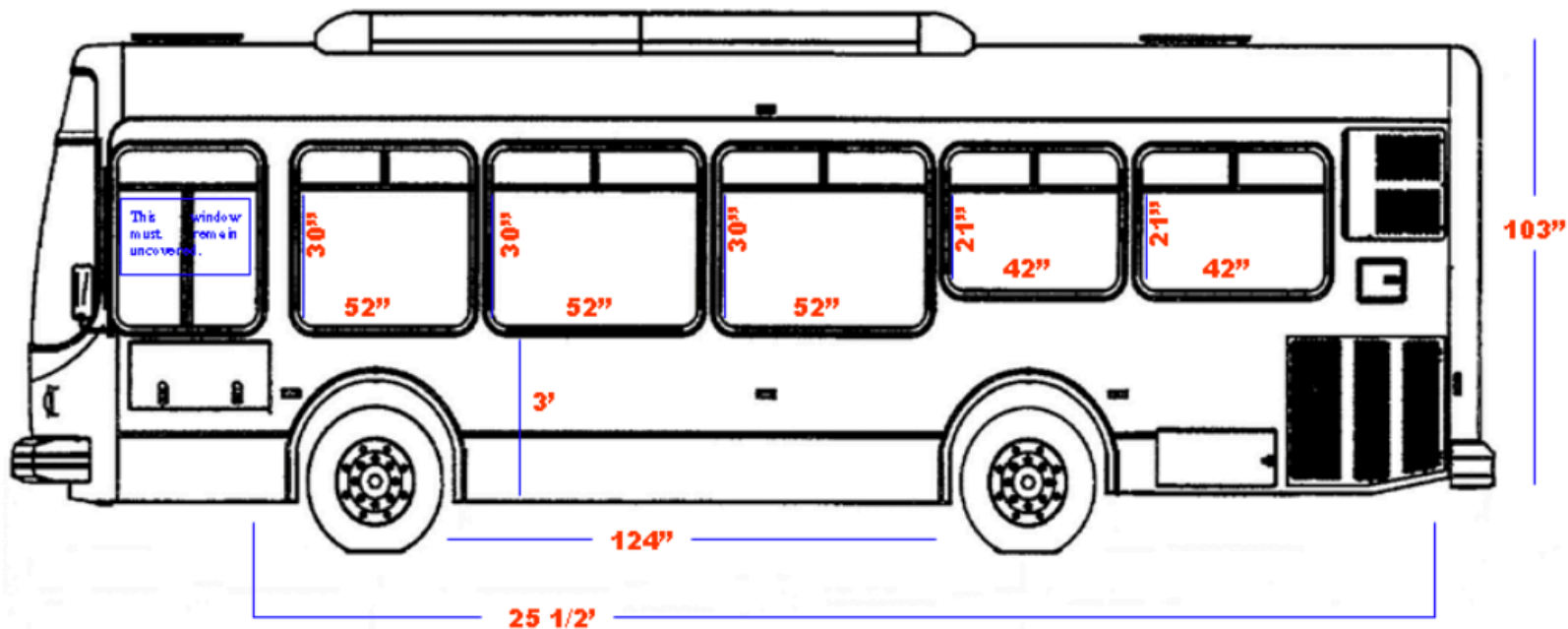
Eldorado Transit Bus:
